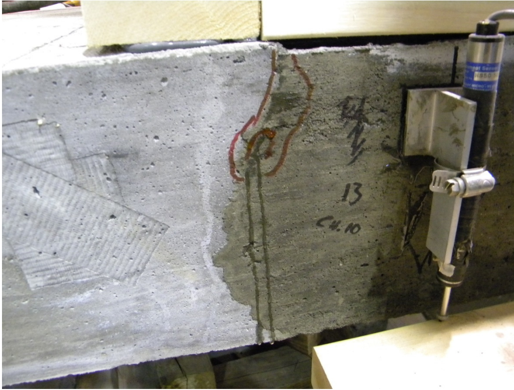
Figure 3.25: Leaking at end of joint
