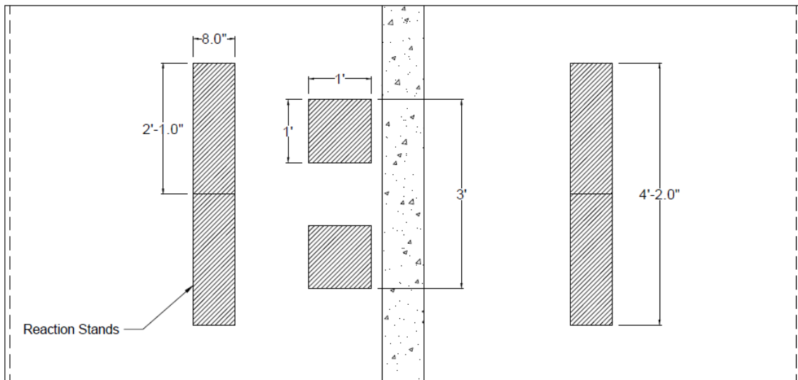
Figure 3.20: Plan view of test set up
